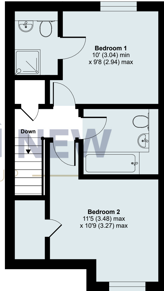
FIRST FLOOR- 402 sq ft / 37.3 sq m
