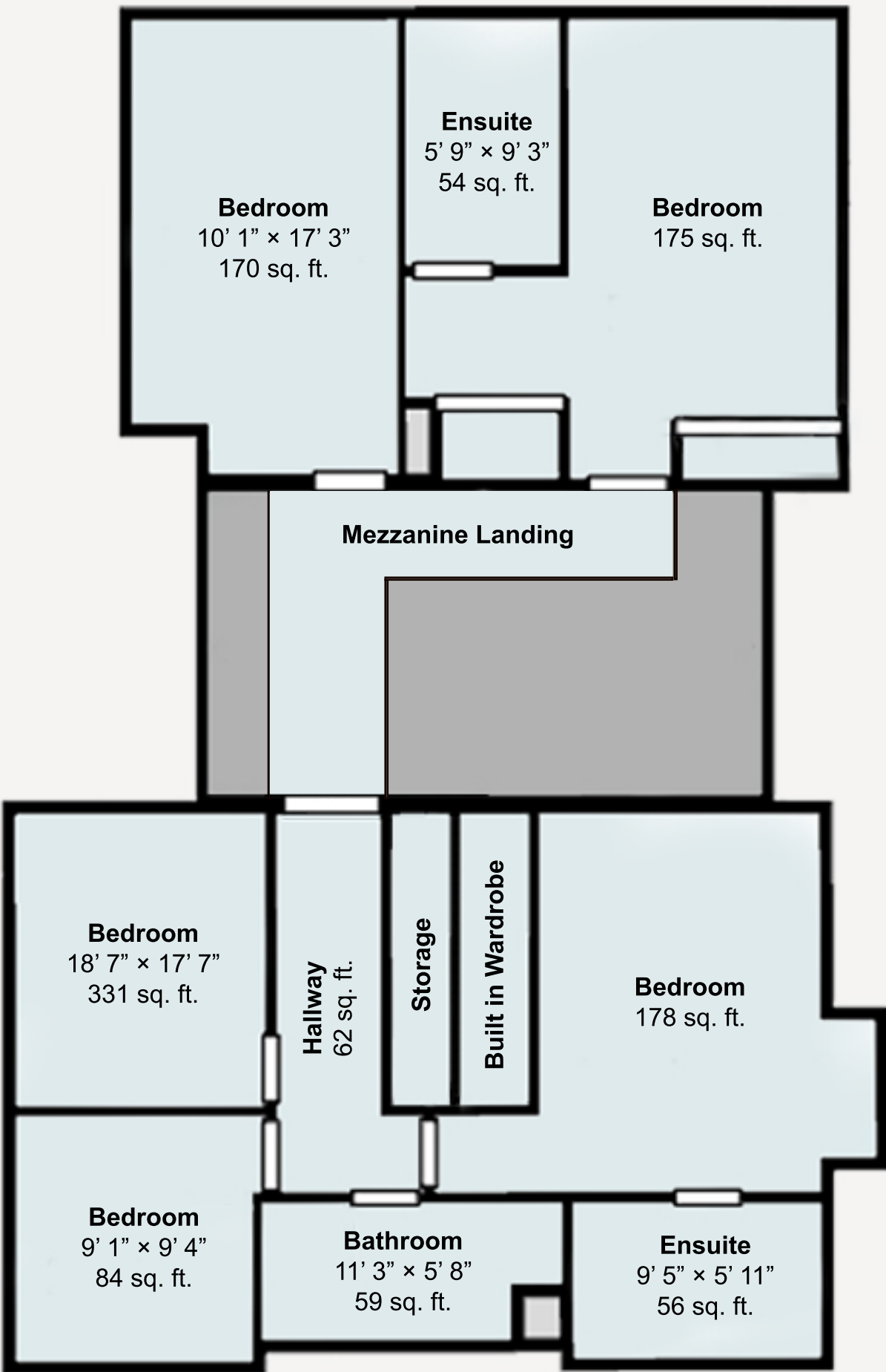
FIRST FLOOR
